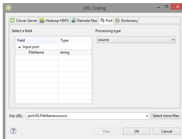
Figure 23.10. URL File Dialog - Clover Server
