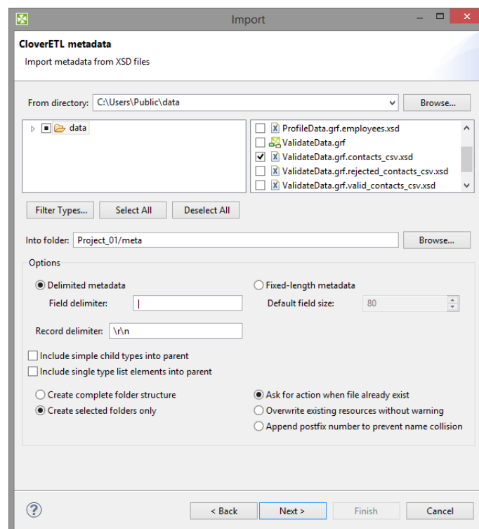
Figure 24.8. Import Metadata from XSD
