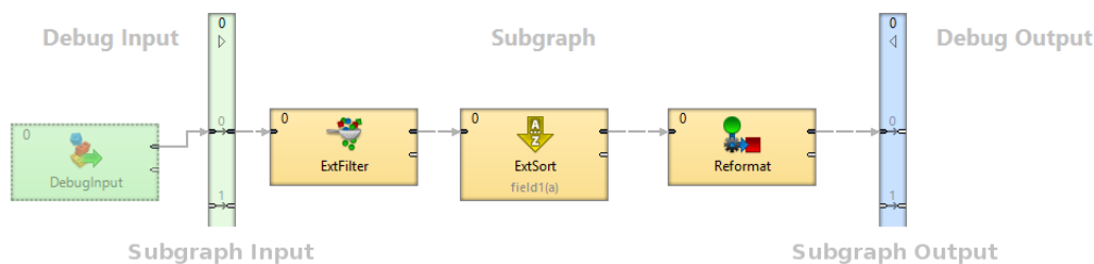
Figure 41.1. Subgraph Layout
