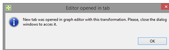
Figure 39.10. Confirmation Message
