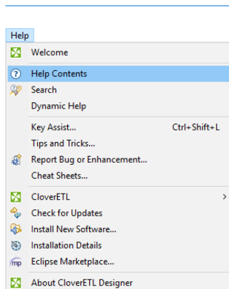
Figure 7.4. CloverETL Help
