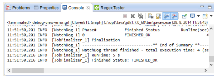
Figure 19.24. Console Tab
