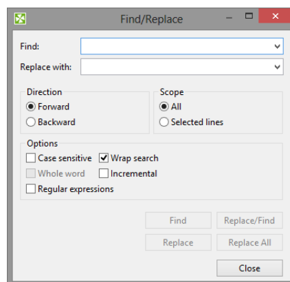
Figure 23.14. Find Wizard
