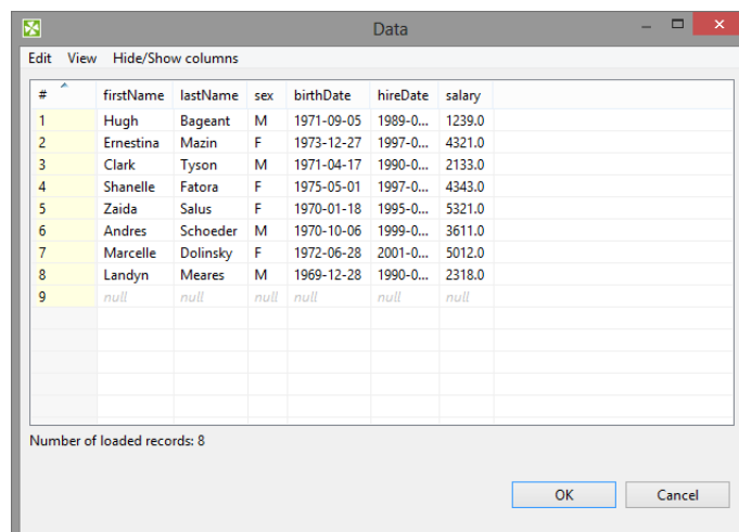
Figure 33.10. Changing Data
