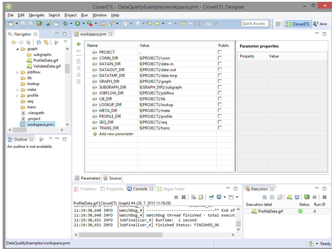
Figure 20.16. Workspace.prm File
