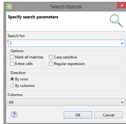
Figure 30.14. Search Options
