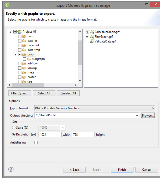
Figure 25.10. Export Image
