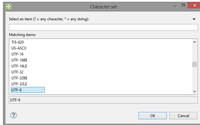
Figure 35.22. Character set
