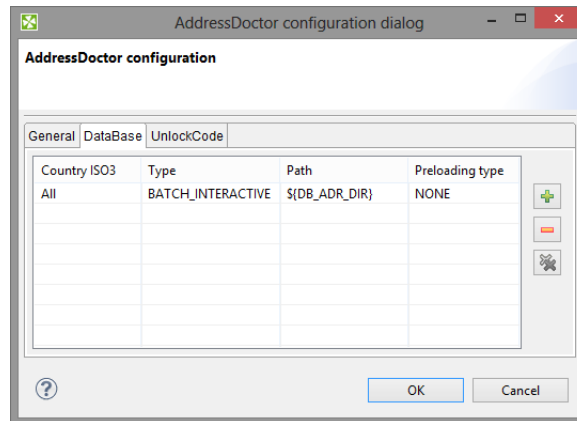
Figure 54.1. DataBase Configuration
