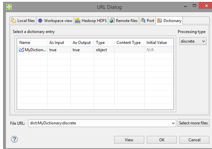
Figure 23.11. URL File Dialog - Dictionary
