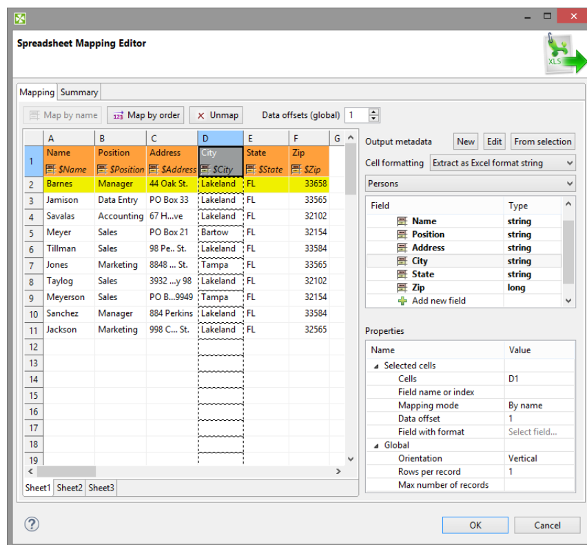
Figure 47.13. Basic Mapping – notice leading cells and dashed borders marking the area data will be taken from
