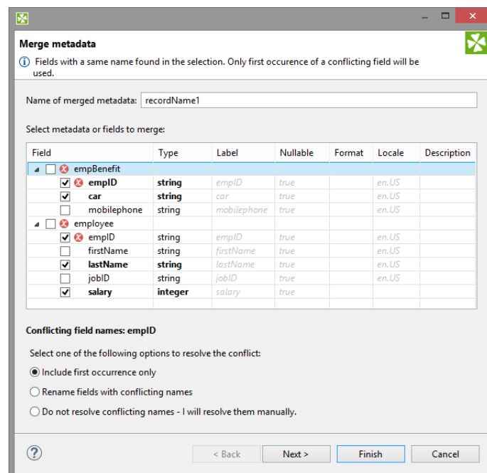
Figure 31.34. Merging two metadata - conflicts can be resolved in one of the three ways (notice radio buttons at the bottom).
