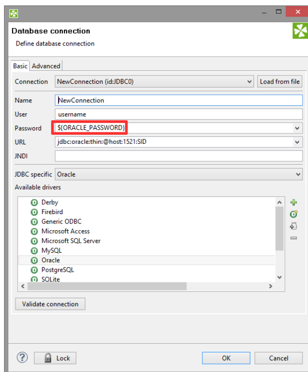
Figure 32.8. Using password from secure graph parameter
