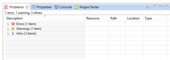
Figure 19.25. Problems Tab
