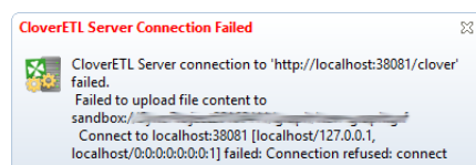
Figure 20.20. Connection failed
