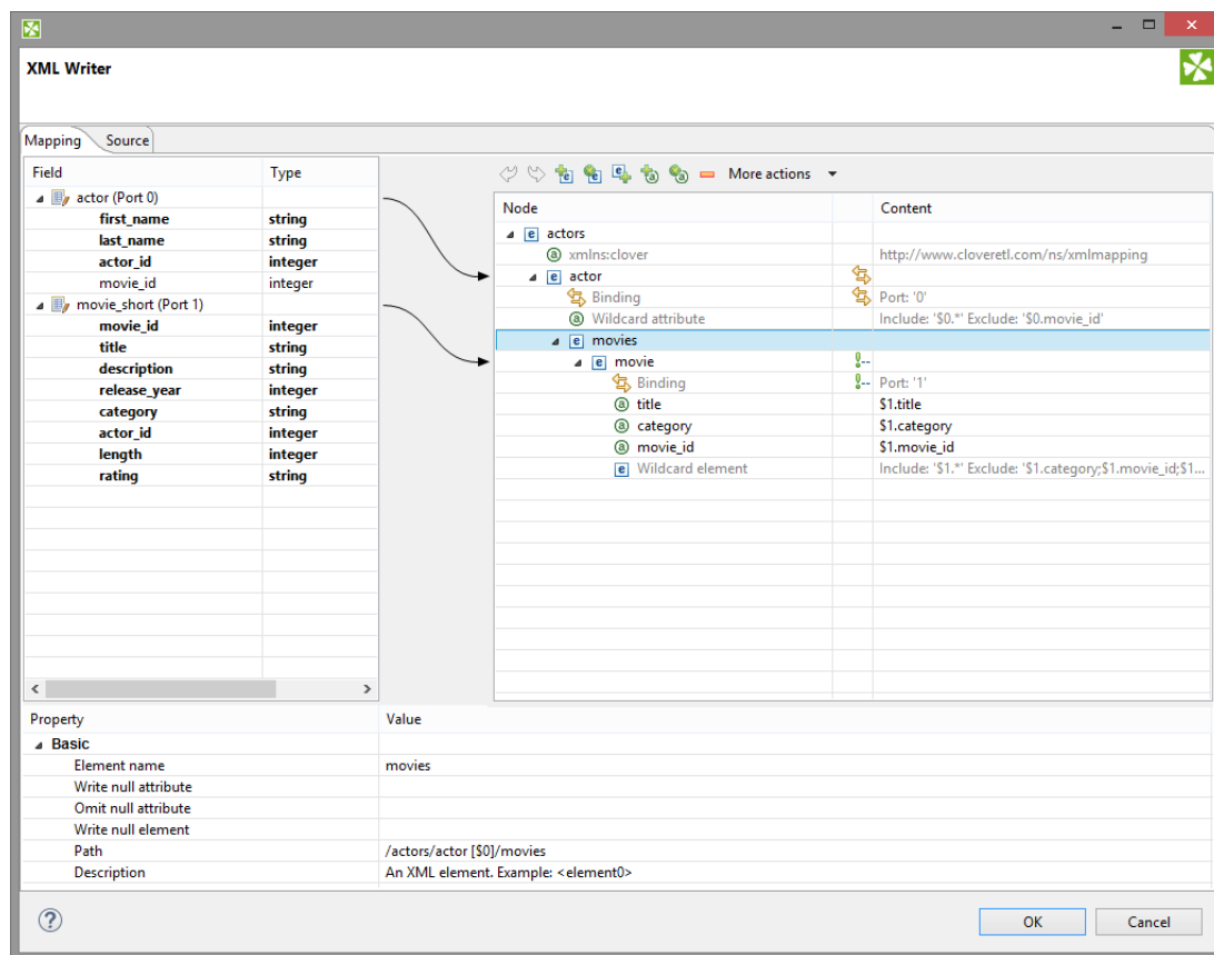
Figure 48.28. Mapping Editor
