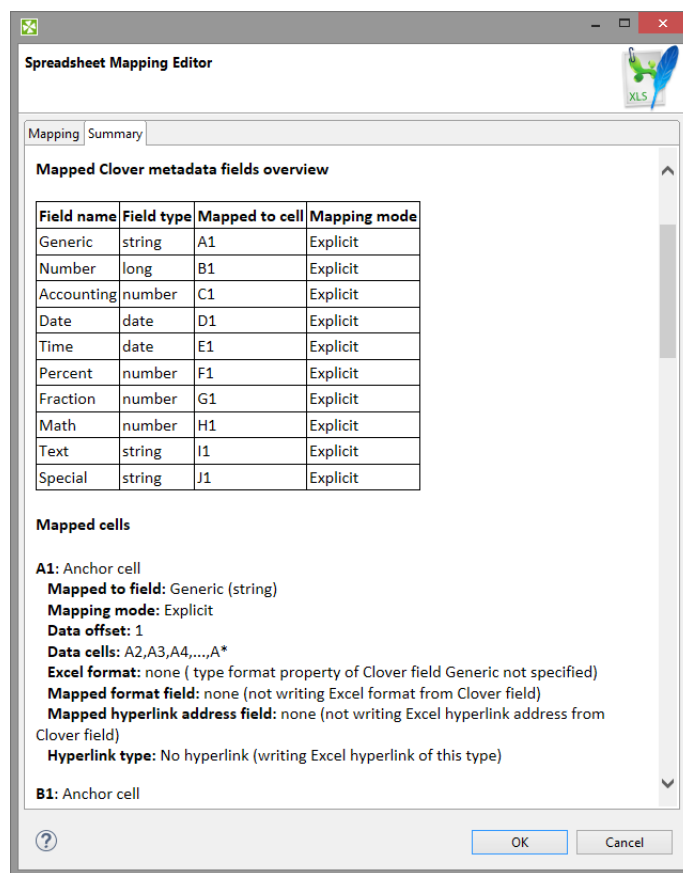
Figure 48.25. Mapping summary
