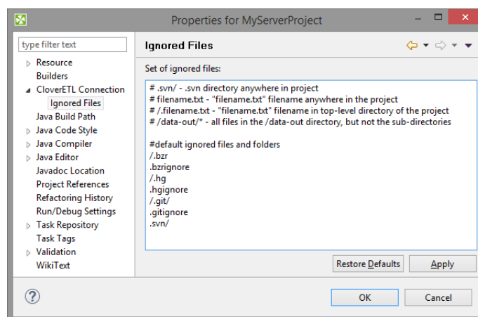
Figure 20.23. CloverETL Connection
