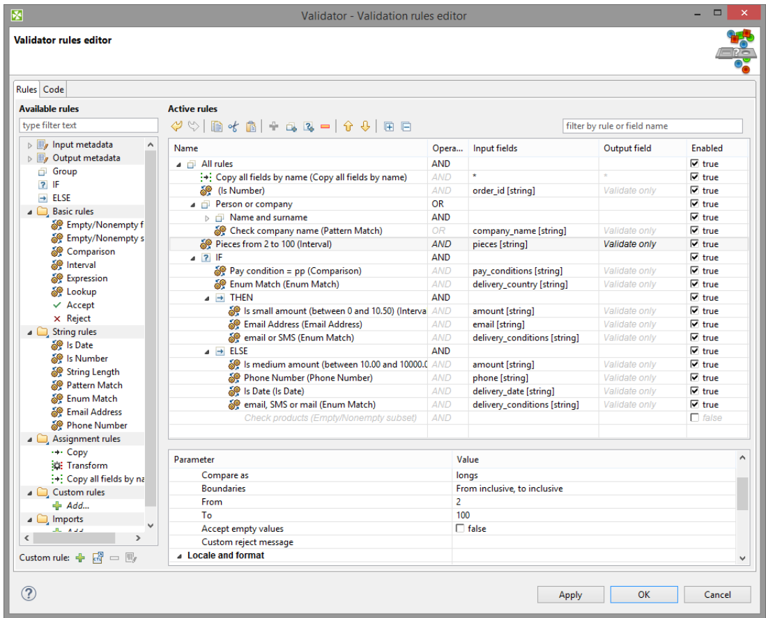
Figure 54.8. Validator rules editor
