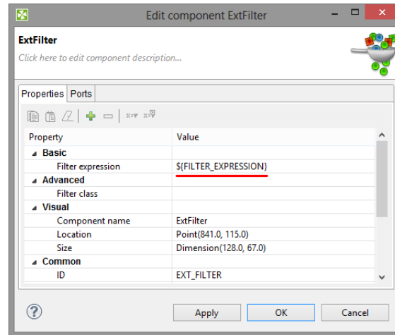
Figure 35.28. Filter Component Configured by Graph Parameter
