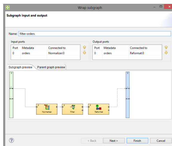
Figure 43.3. Wrapping Subgraph Wizard
