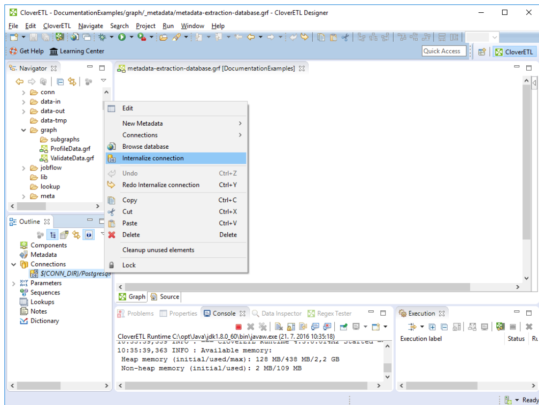
Figure 32.3. Internalizing External (Shared) Database Connection
