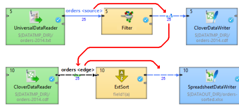
Figure 31.16. Metadata propagated from an unconnected distant edge
