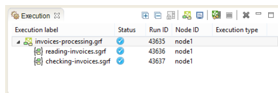
Figure 19.28. Execution tab of a graph running on CloverETL Server
