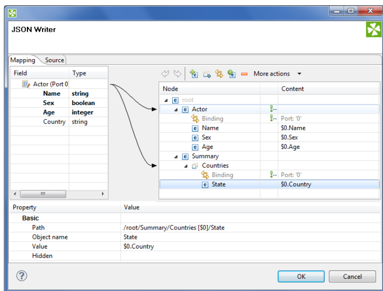
Figure 48.16. Mapping arrays in JSONWriter - notice the array contains a dummy element 'State' which you bind the input field to.
