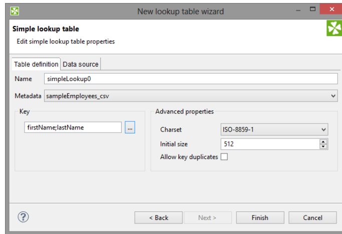
Figure 33.6. Simple Lookup Table Wizard
