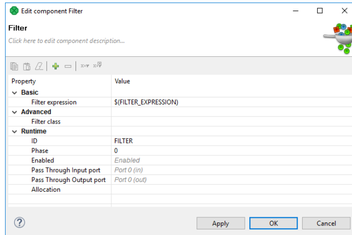
Figure 37.26. Filter Component Configured by Graph Parameter
