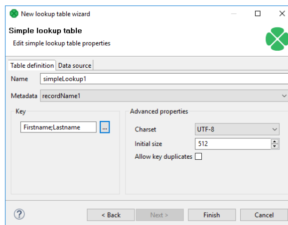
Figure 35.2. Simple Lookup Table Wizard
