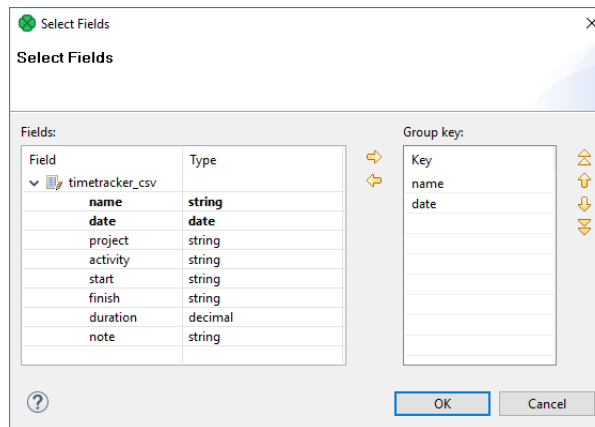
Figure 31.10. Defining Group Key
