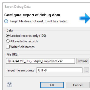
Figure 32.9. Export Debug Data to CSV
