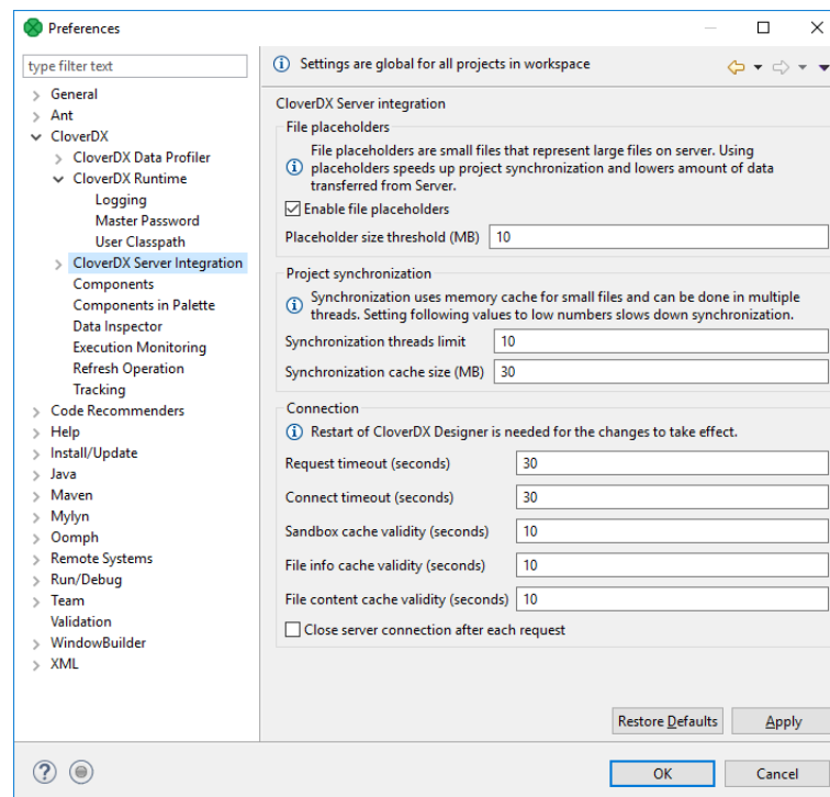
Figure 16.1. CloverDX Server Integration
