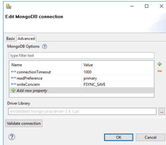
Figure 34.13. MongoDB Connection Dialog - Advanced Tab
