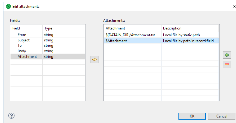
Figure 57.5. Edit Attachments Wizard
