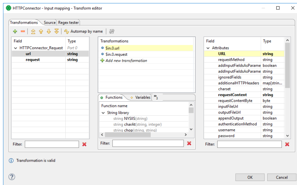
Figure 64.4. Transform Editor in HTTPConnector
