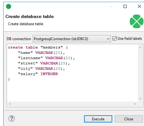
Figure 33.31. Creating Database Table from Metadata and Database Connection
