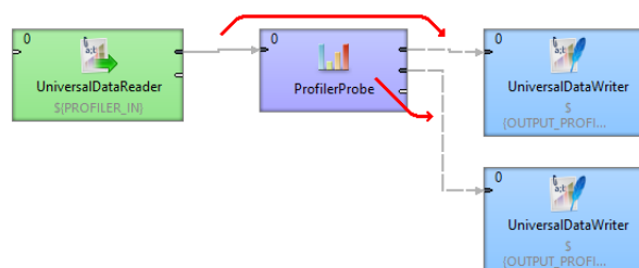
Figure 33.7. Metadata propagated from the component, metadata template is defined within the component.
