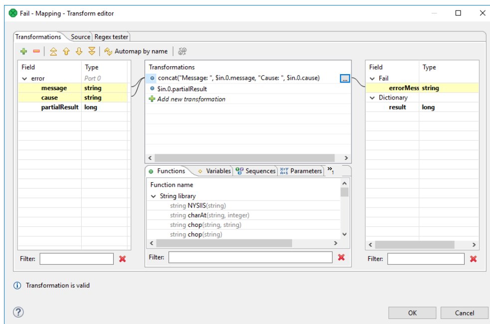
Figure 60.2. Example of mapping for the Fail component
