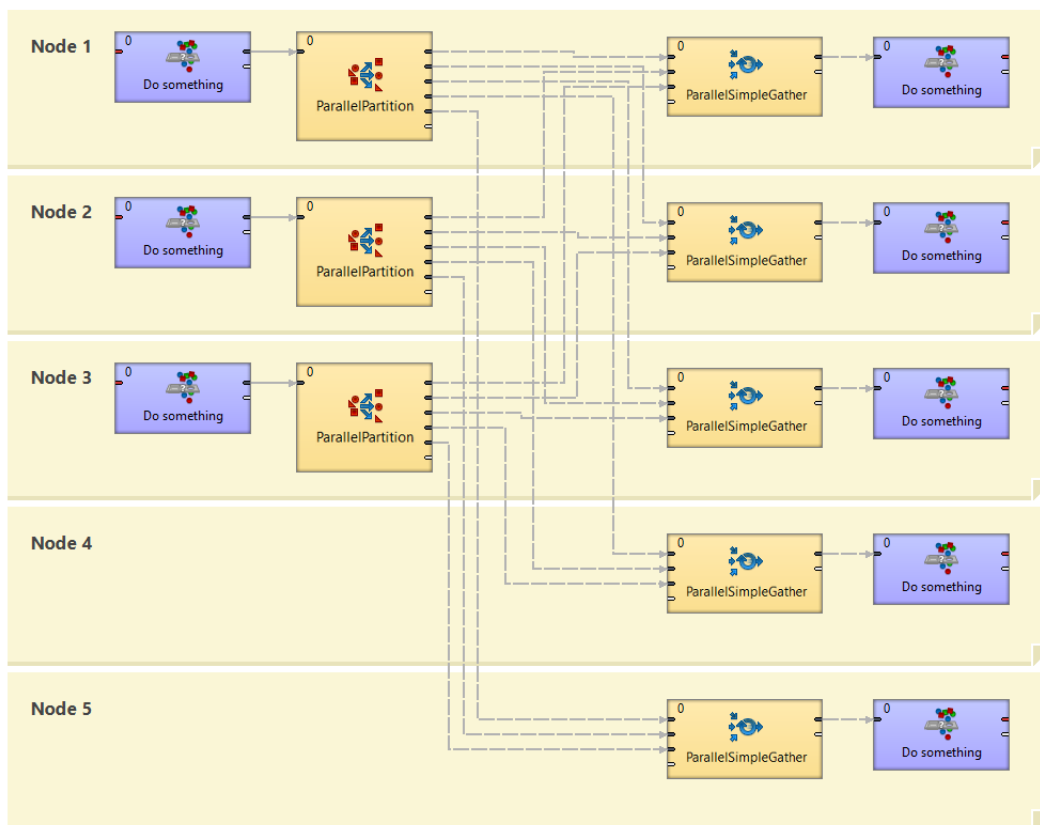
Figure 62.2. Example of actual working of ParallelRepartition component in runtime
