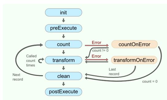
Figure 58.3. Normalizer code workflow
