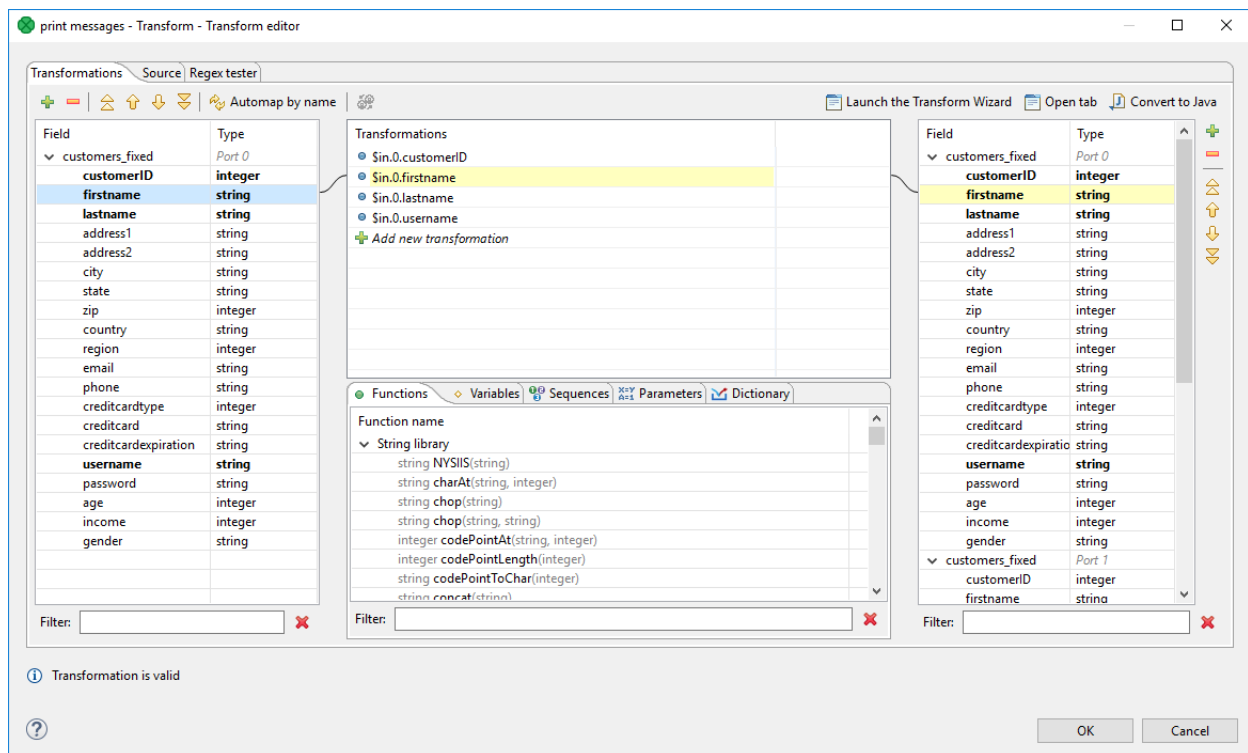
Figure 41.2. Transformations Tab of the Transform Editor
