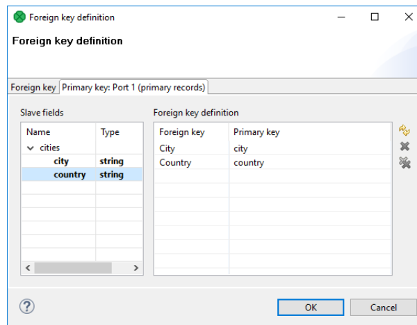
Figure 64.3. Foreign Key Definition Wizard (Foreign and Primary Keys Assigned)
