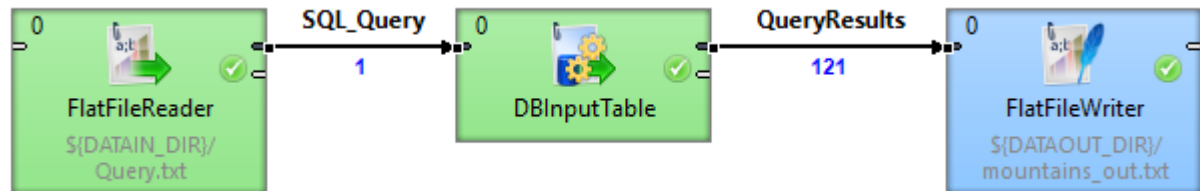
Figure 56.9. Reading query from input port
