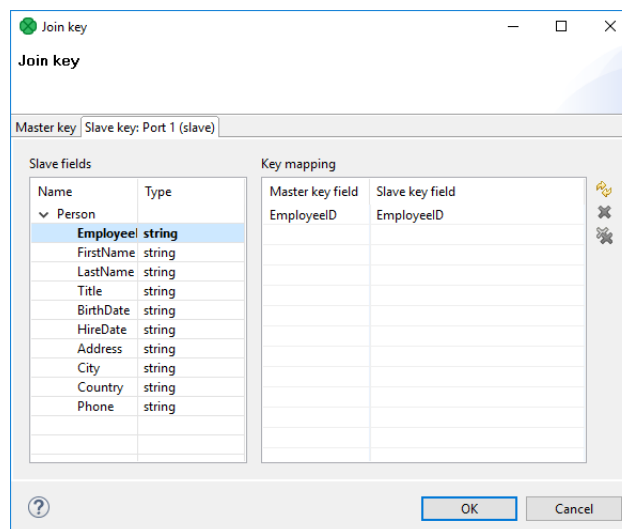
Figure 59.4. Join Key Wizard (Slave Key Tab)
