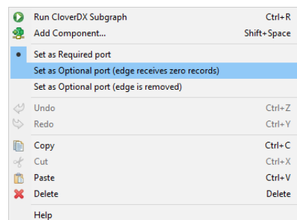
Figure 46.10. Setting up an Optional Port in Graph Editor
