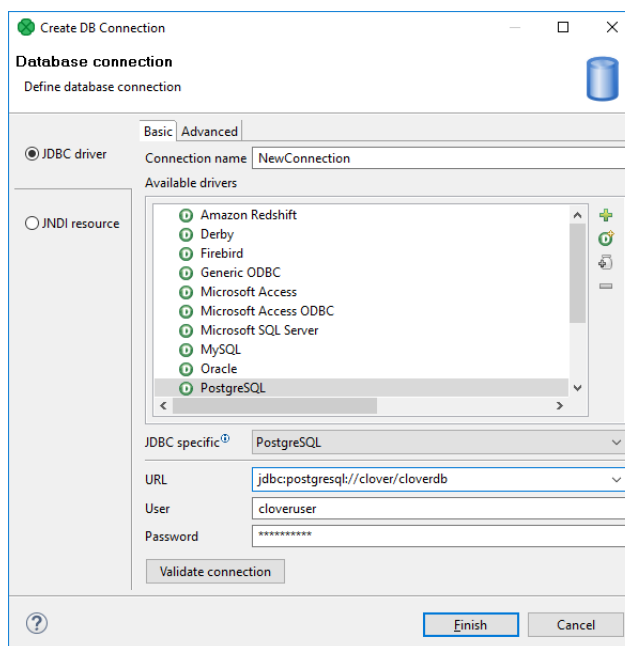
Figure 34.1. Database Connection Properties Dialog
