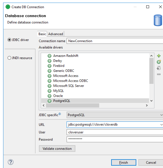
Figure 33.21. Database Connection Properties Dialog
