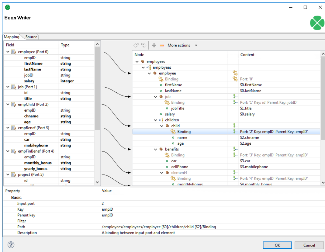
Figure 57.9. Example mapping in JavaBeanWriter
