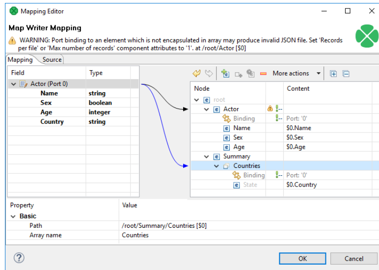
Figure 57.12. Mapping arrays in JavaMapWriter - notice the array contains a dummy element 'State' which you bind the input field to.
