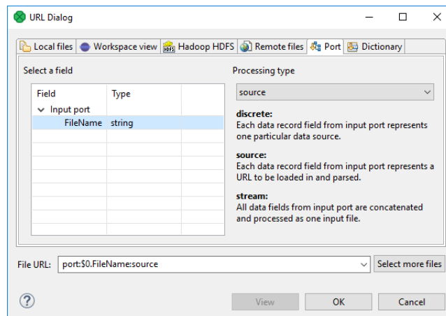
Figure 25.7. URL File Dialog - Input Port
