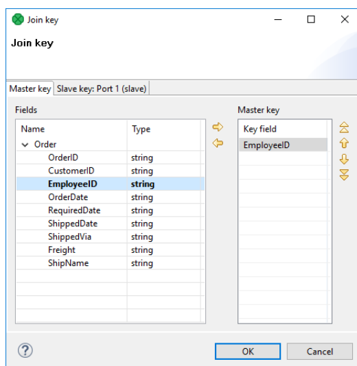
Figure 59.9. Join Key Wizard (Master Key Tab)
