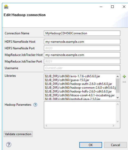
Figure 34.11. Hadoop Connection Dialog
