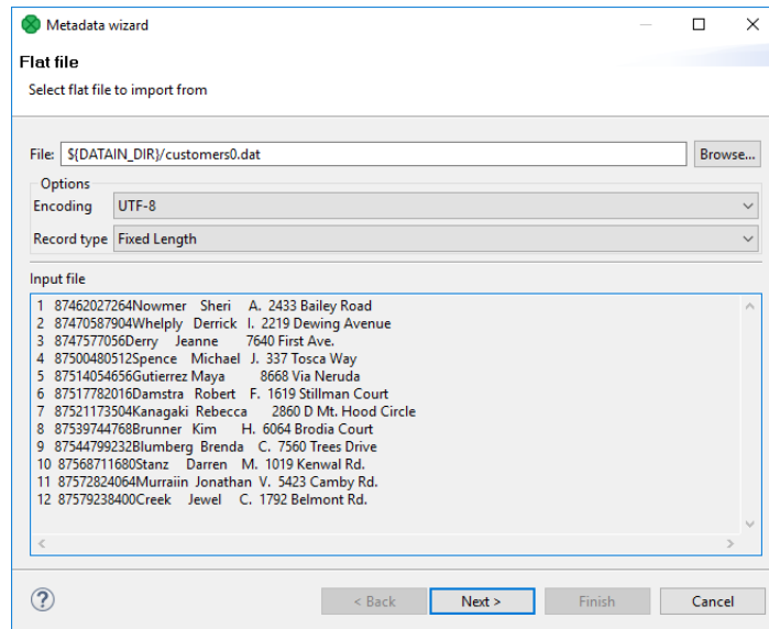
Figure 33.15. Extracting Metadata from Fixed Length Flat File
