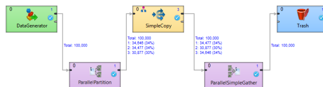
Figure 28.2. An example of a medium level of tracking information
