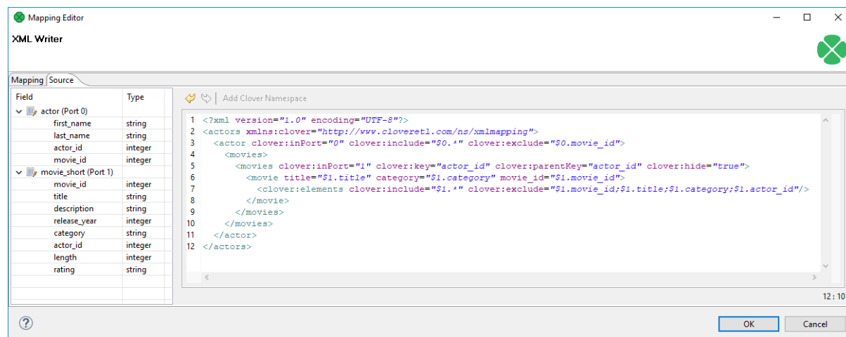
Figure 57.35. Source tab in Mapping editor
