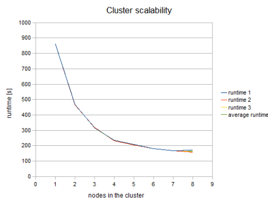
Figure 43.7. Cluster Scalability
