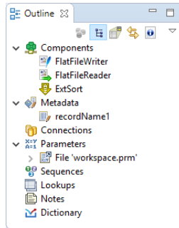
Figure 21.5. Outline Pane
