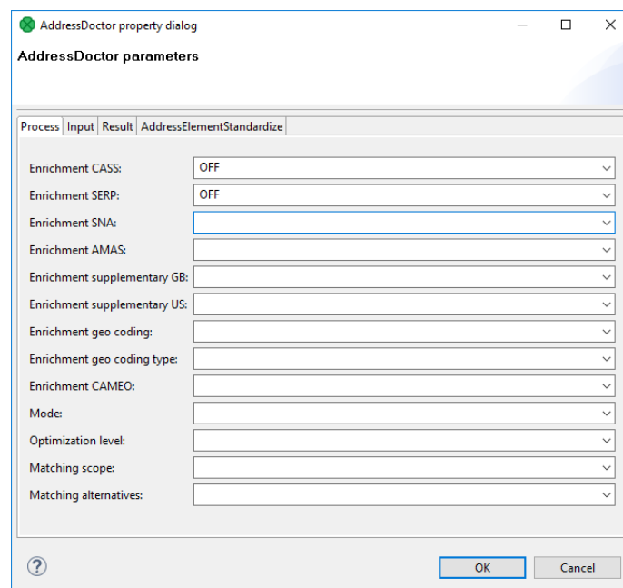
Figure 63.2. AddressDoctor Parameters
