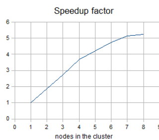
Figure 43.8. Speedup factor
