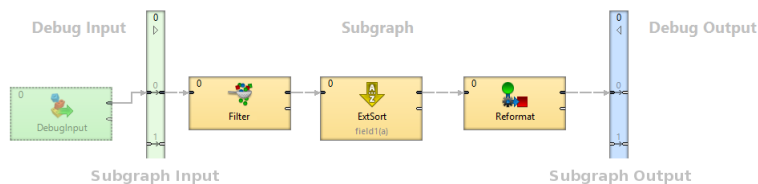
Figure 44.1. Subgraph Layout
