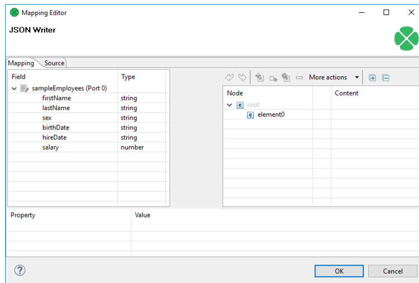
Figure 57.13. Mapping editor in JSONWriter after first open. Metadata on the input edge(s) are displayed on the left hand side. The right hand pane is where you design the desired JSON tree. Mapping is then performed by dragging metadata from left to right (and performing additional tasks described below).
