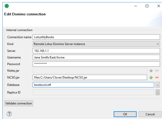
Figure 34.10. Lotus Notes Connection Dialog
