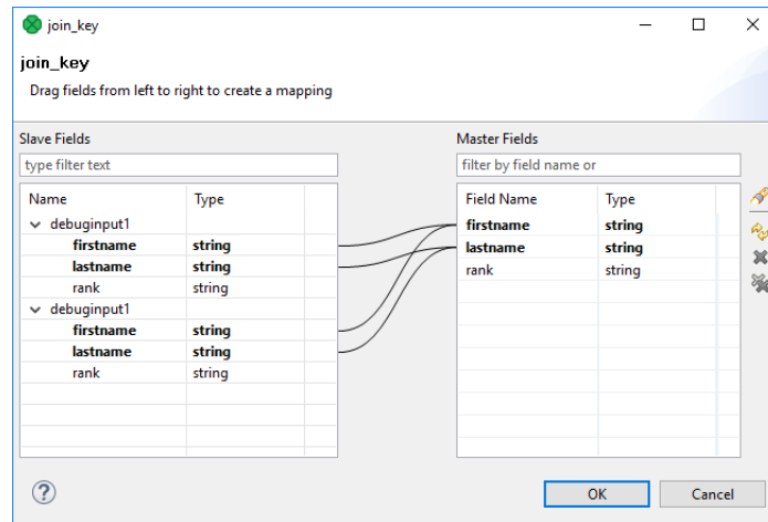
Figure 37.19. Join Key - Configuration
