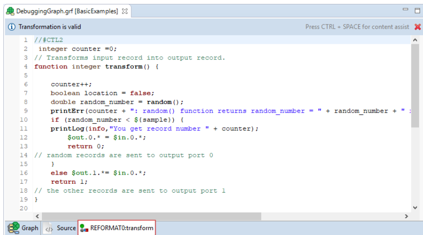
Figure 41.10. Transformation Definition in CTL (Transform Tab of the Graph Editor)
