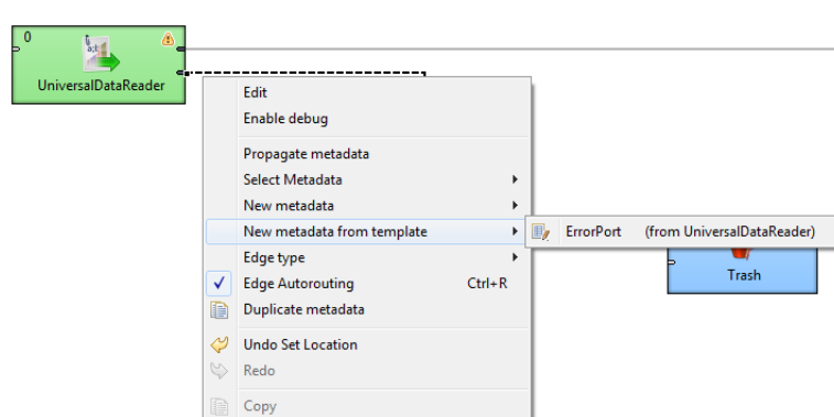
Figure 31.12. Creating Metadata from a Template
