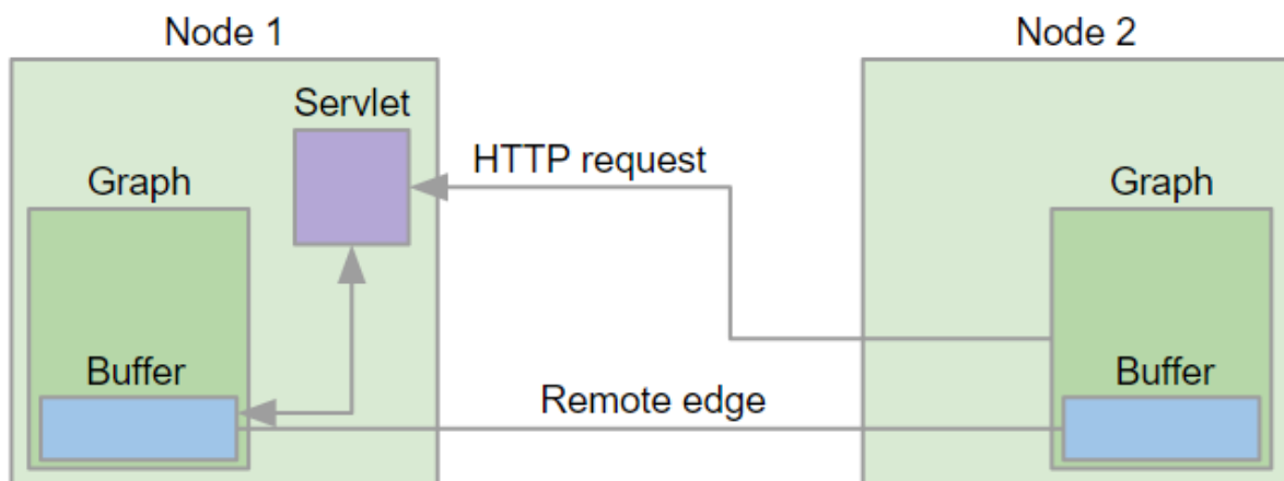
Figure 43.9. Remote Edge Implementation
