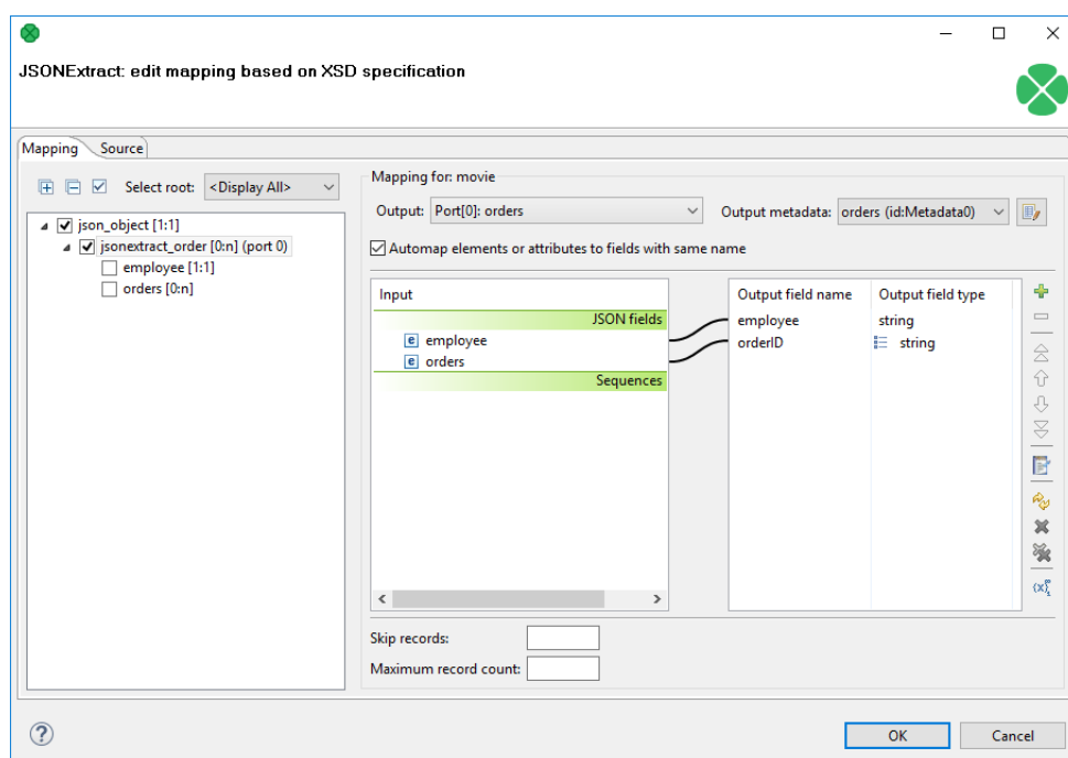
Figure 56.15. JSONExtract - mapping the list
