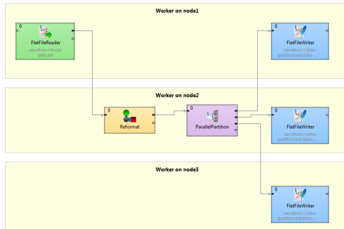
Figure 43.2. Graph decomposition based on component allocations
