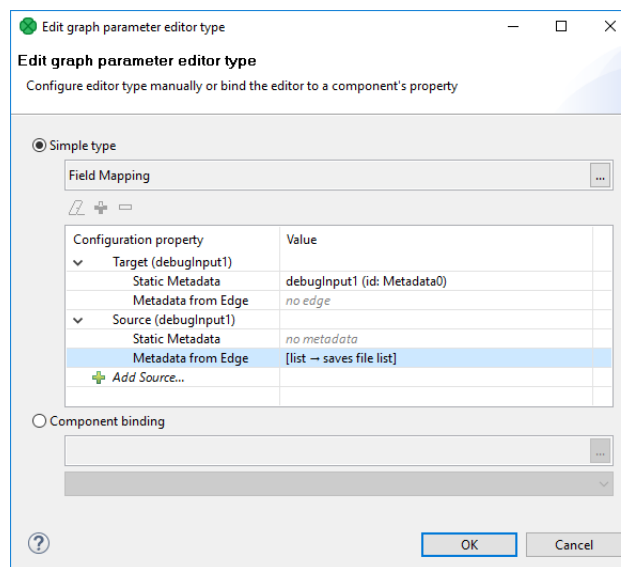
Figure 37.16. Field Mapping - Configuration
