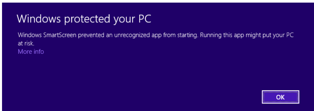
Figure 13.1. SmartScreen warning
