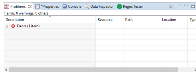
Figure 21.14. Problems Tab
