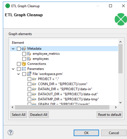
Figure 21.9. Graph Cleanup
