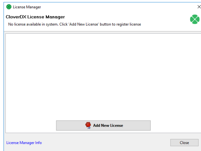
Figure 9.6. License Manager
