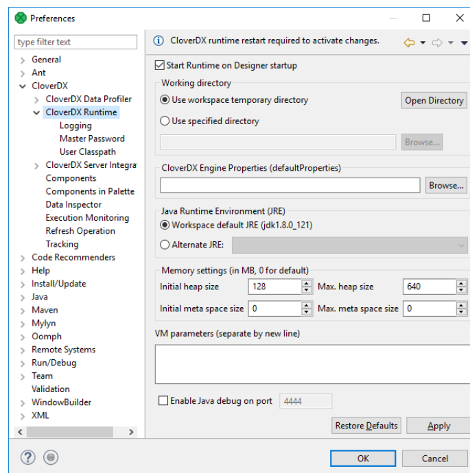
Figure 15.1. CloverDX Runtime
