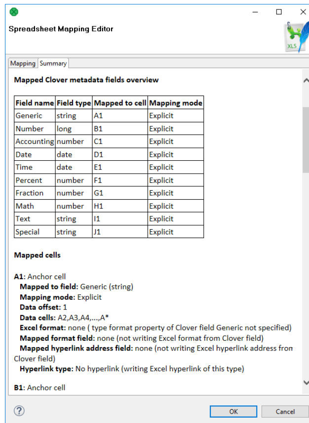
Figure 57.24. Mapping summary
