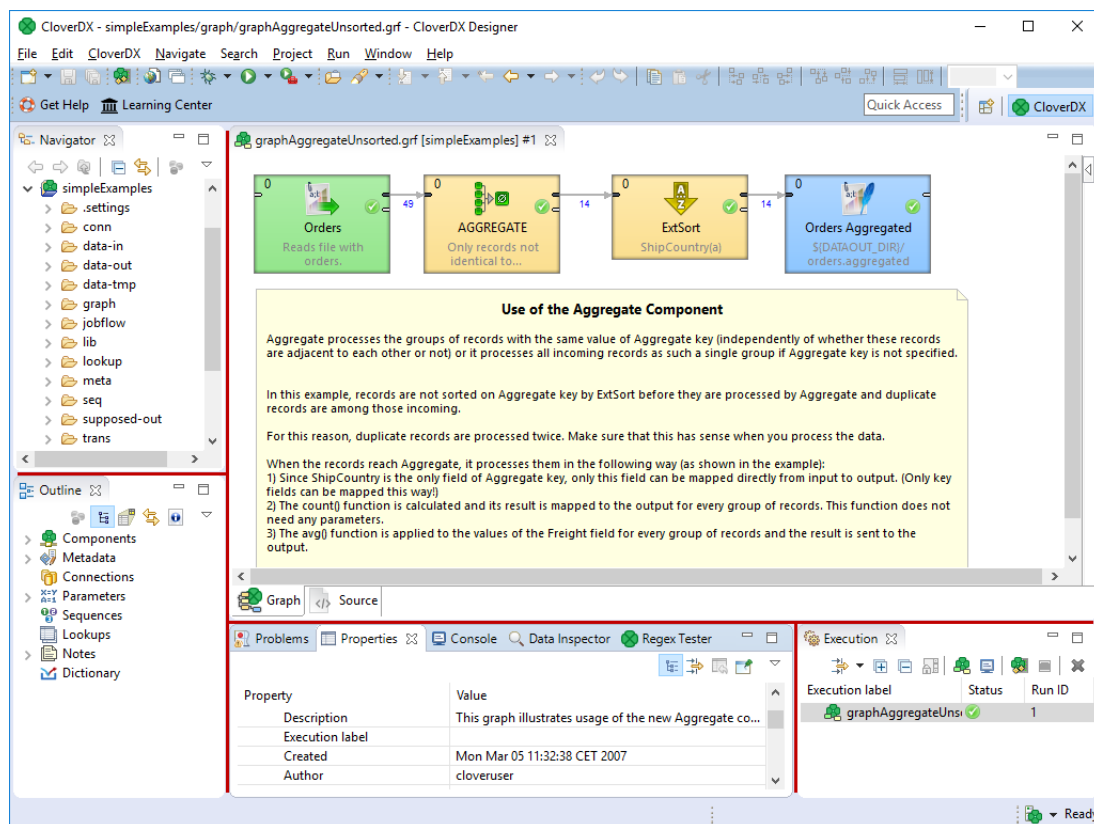
Figure 21.1. CloverDX Perspective
