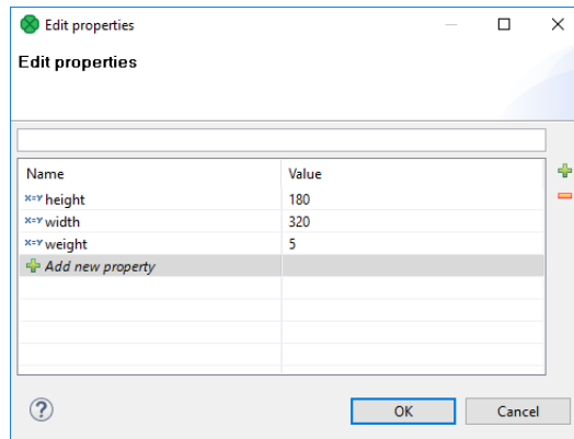
Figure 37.11. Properties - Usage
