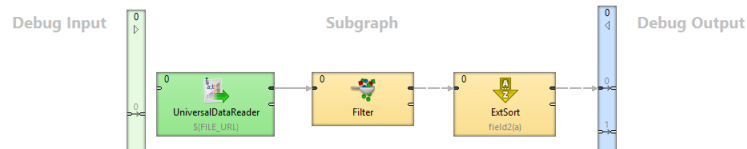
Figure 47.1. Subgraph - Reader
