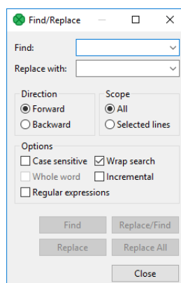
Figure 25.11. Find Wizard
