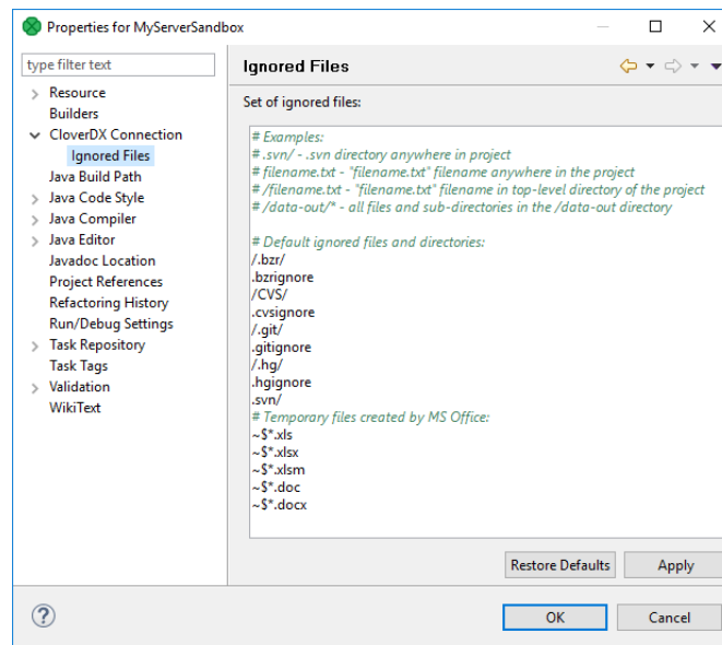
Figure 22.17. CloverDX Connection
