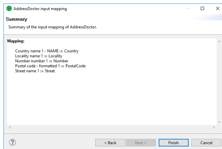
Figure 63.4. Input mapping wizard
