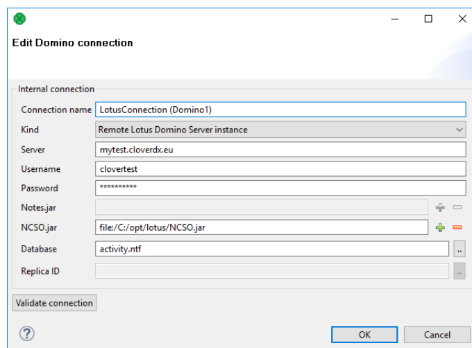
Figure 33.28. Specifying Lotus Notes connection for metadata extraction
