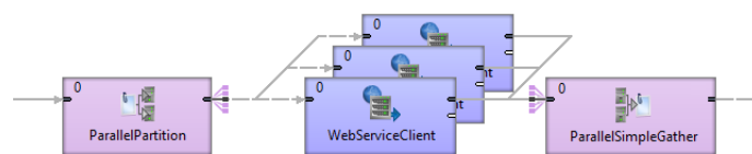
Figure 42.1. Illustration of Parallel Run
