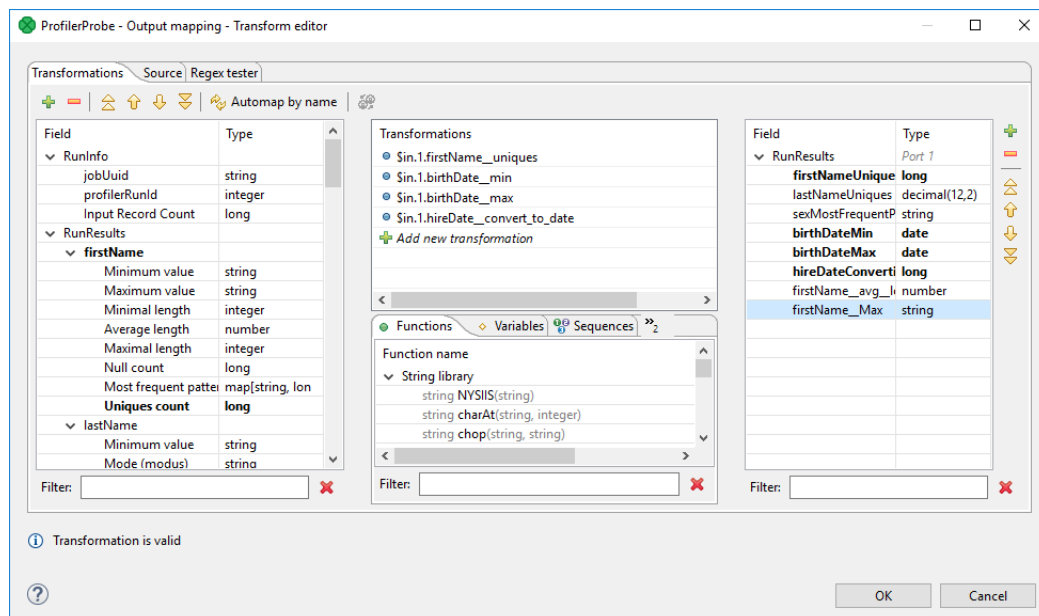
Figure 63.6. Transform Editor in ProfilerProbe
