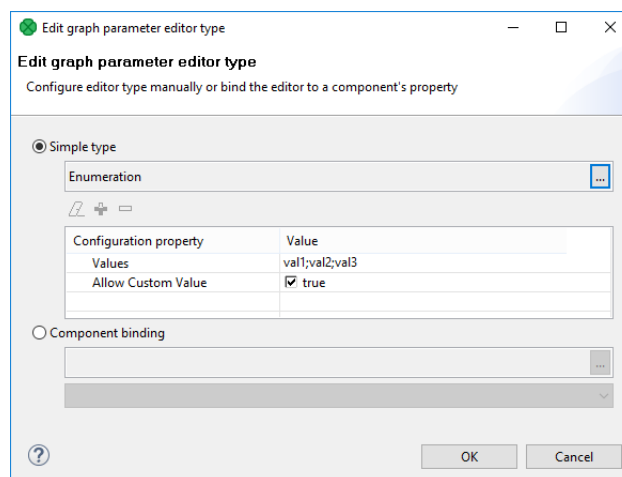
Figure 37.20. Enumeration - Configuration
