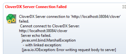
Figure 22.13. Connection failed
