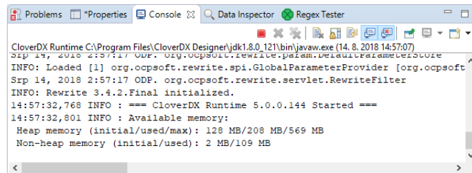
Figure 21.13. Console Tab
