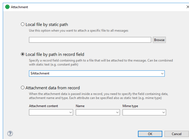
Figure 57.6. Attachment Wizard
