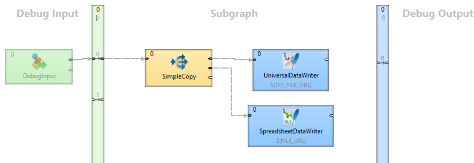
Figure 47.2. Subgraph - Writer
