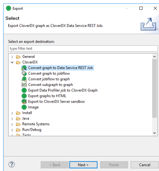
Figure 27.1. Export Options
