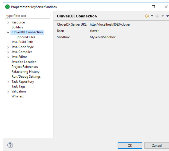
Figure 22.16. CloverDX Connection
