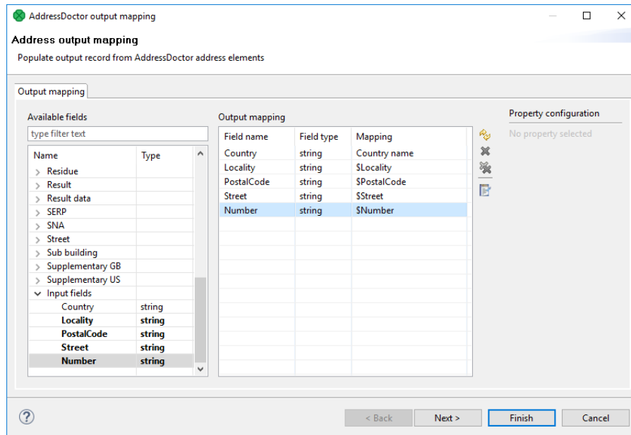
Figure 63.5. Output mapping
