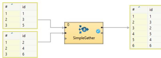
Figure 58.5. SimpleGather
