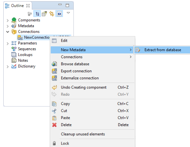
Figure 33.20. Extracting Internal Metadata from a Database
