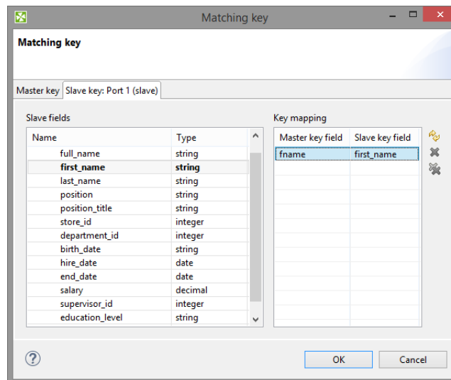
Figure 65.5. Matching Key Wizard (Slave Key Tab)
