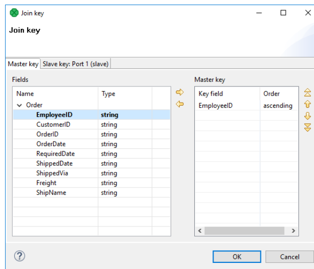
Figure 59.3. Join Key Wizard (Master Key Tab)
