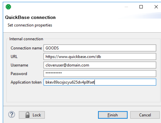
Figure 34.9. QuickBase Connection Dialog
