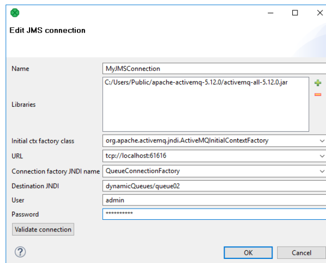
Figure 34.8. Edit JMS Connection Wizard
