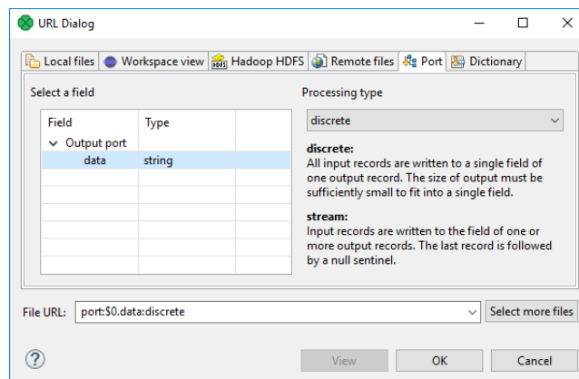
Figure 25.8. URL File Dialog - Output Port
