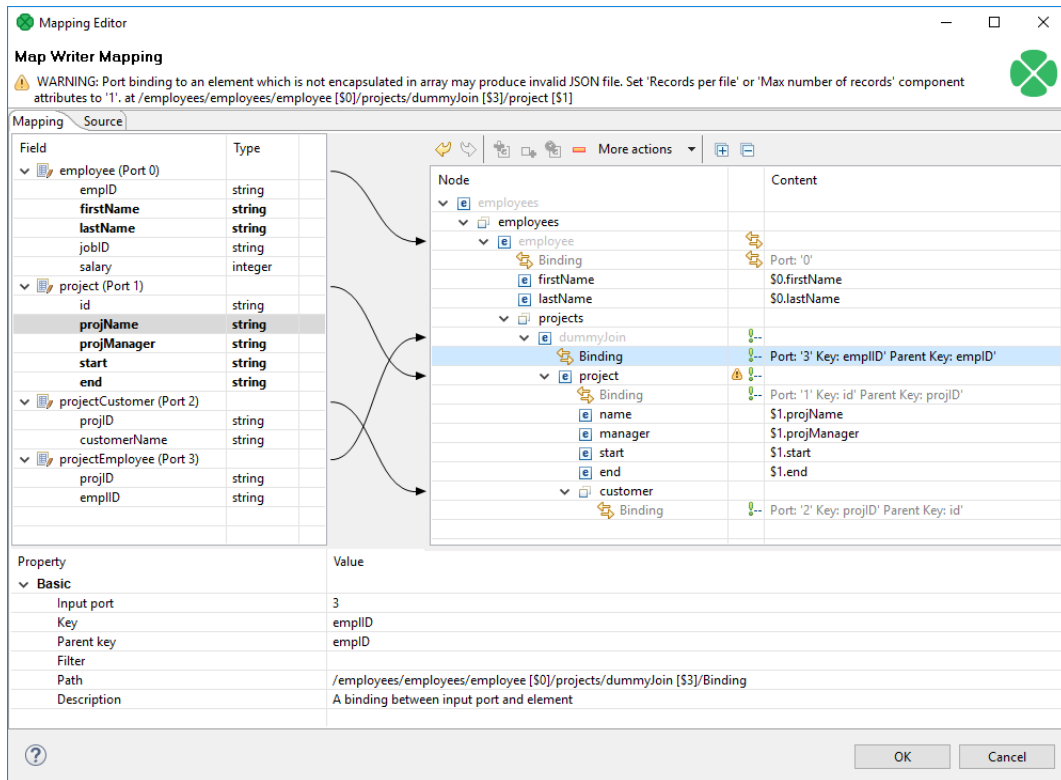
Figure 57.11. Example mapping in JavaMapWriter
