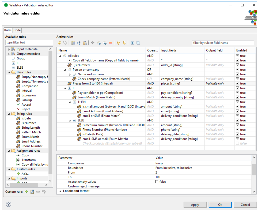
Figure 63.8. Validator rules editor
