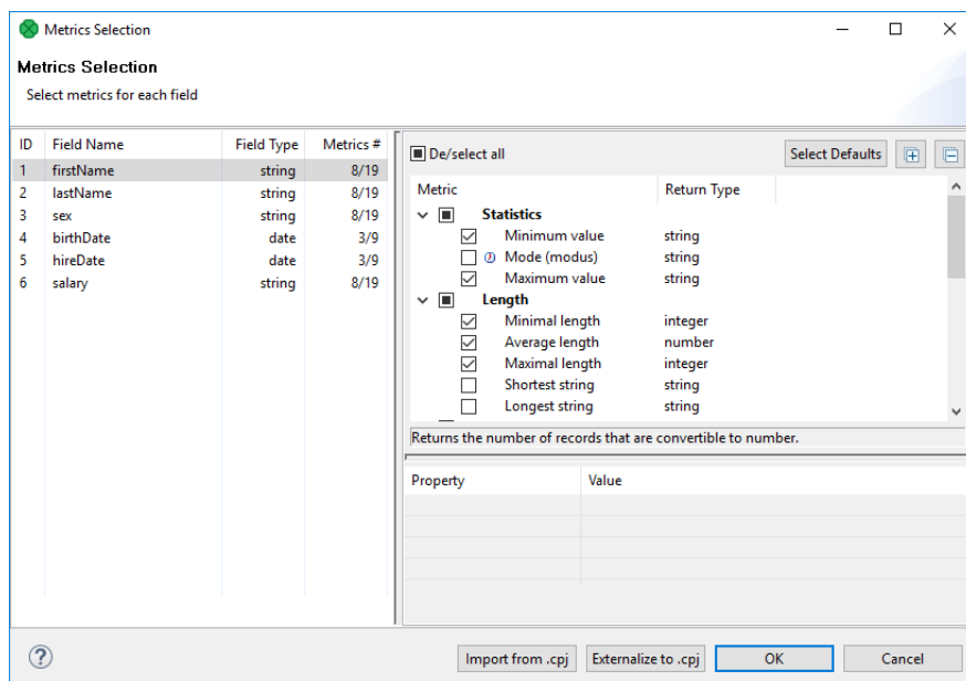
Figure 63.7. Import/Externalize metrics buttons
