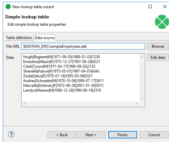
Figure 35.5. Simple Lookup Table Wizard with Data
