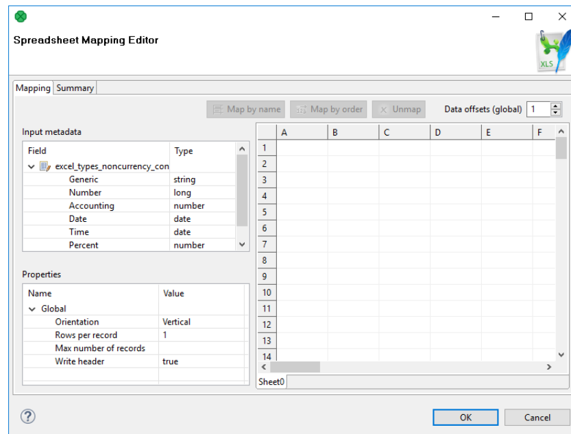
Figure 57.16. Spreadsheet Mapping Editor
