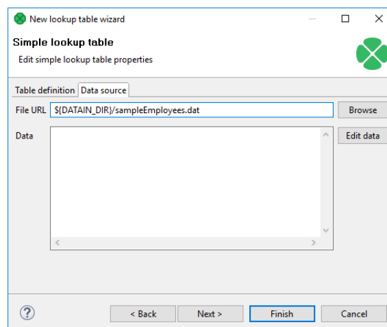
Figure 35.4. Simple Lookup Table Wizard with File URL
