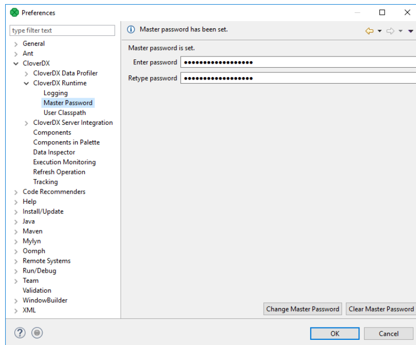
Figure 15.6. Setting the Master password
