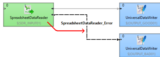
Figure 33.5. Metadata propagated from the component
