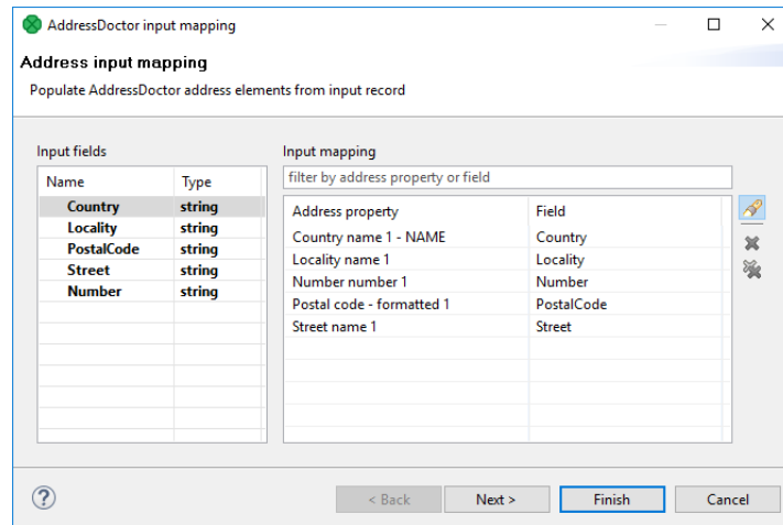
Figure 63.3. Input mapping wizard
