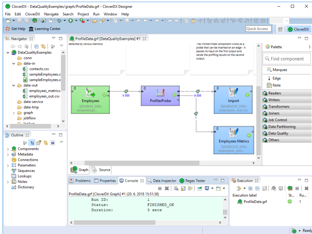
Figure 1.1. CloverDX Designer
