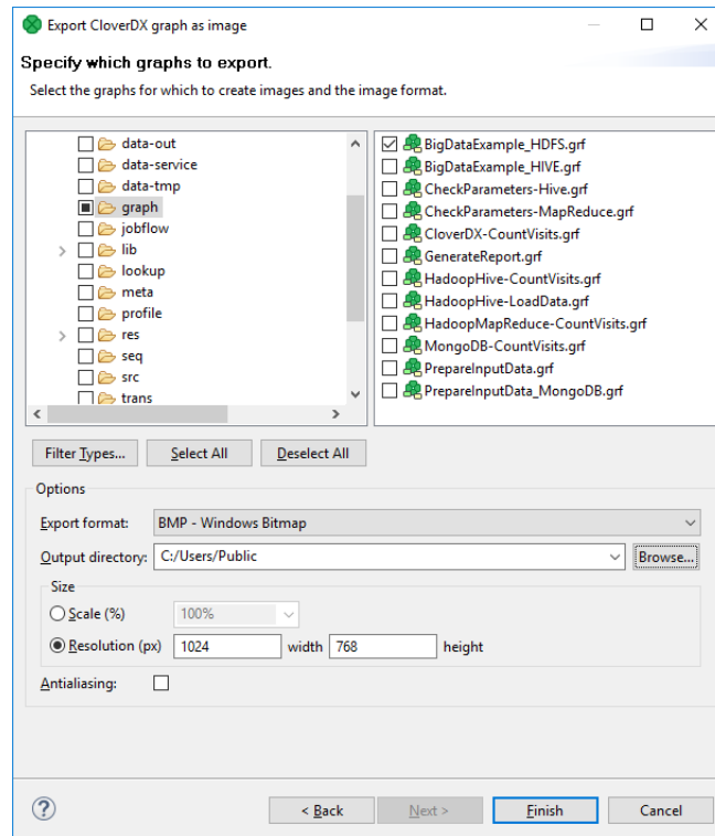
Figure 27.7. Export Image
