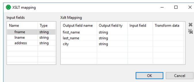
Figure 58.6. XSLT Mapping
