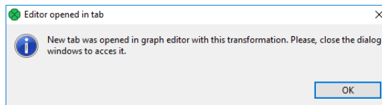
Figure 41.9. Confirmation Message
