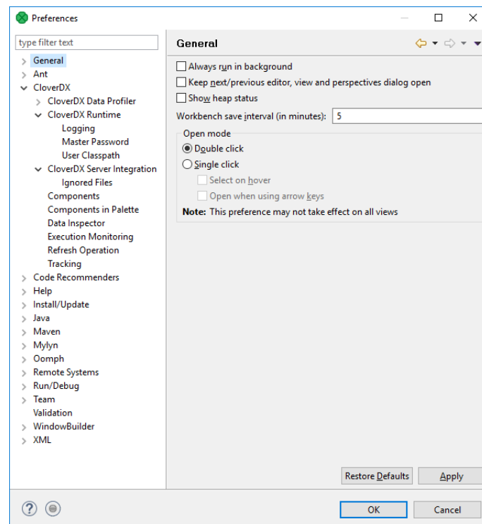
Figure 18.1. Preference Wizard
