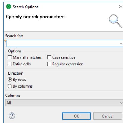
Figure 32.8. Search Options
