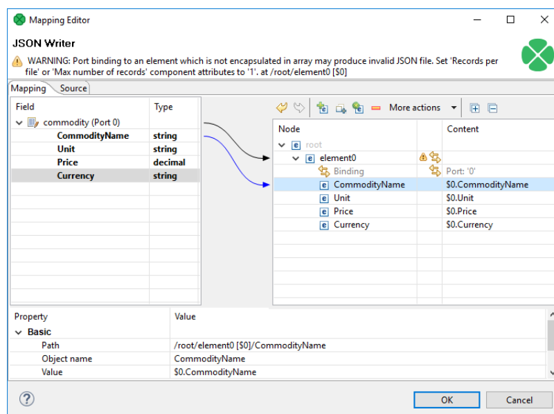
Figure 57.15. JSONWriter mapping
