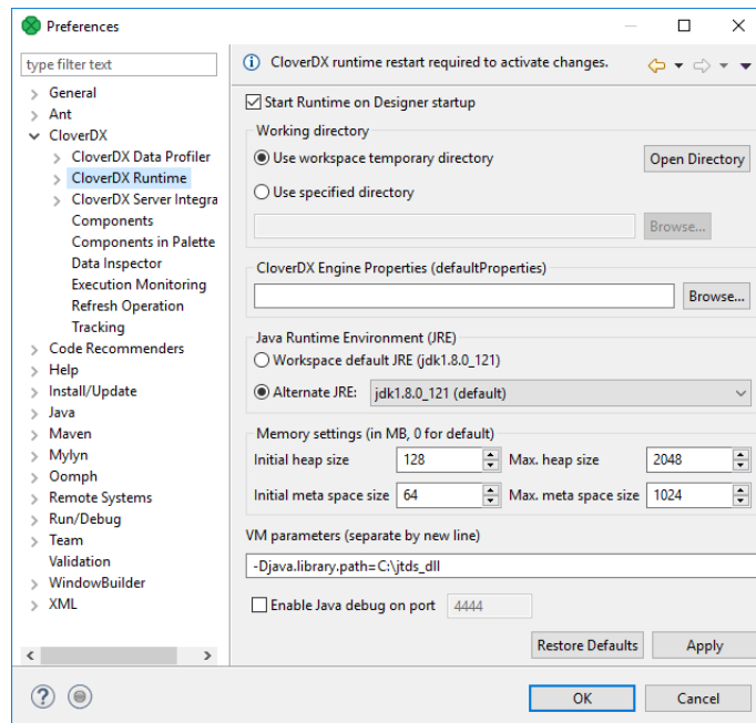
Figure 34.7. Adding path to the native dll to VM parameters.
