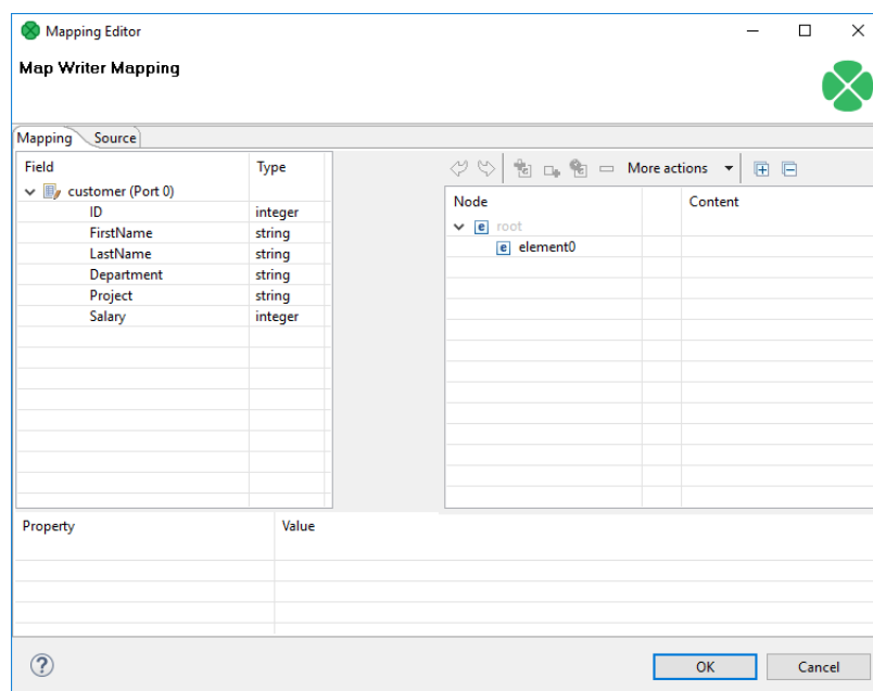
Figure 57.10. Mapping editor in JavaMapWriter after first open.
