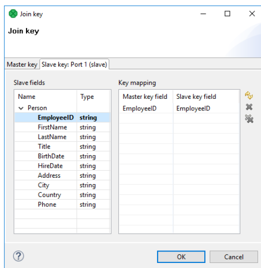
Figure 59.10. Join Key Wizard (Slave Key Tab)
