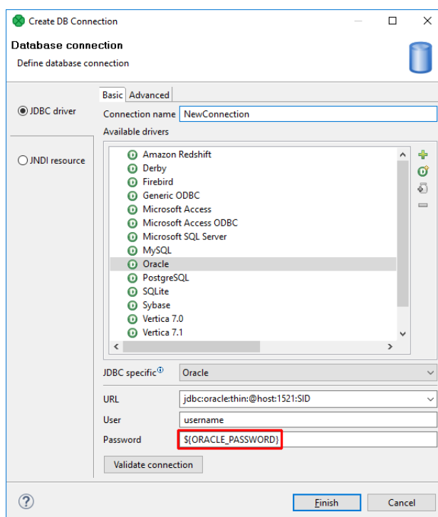
Figure 34.5. Using password from secure graph parameter
