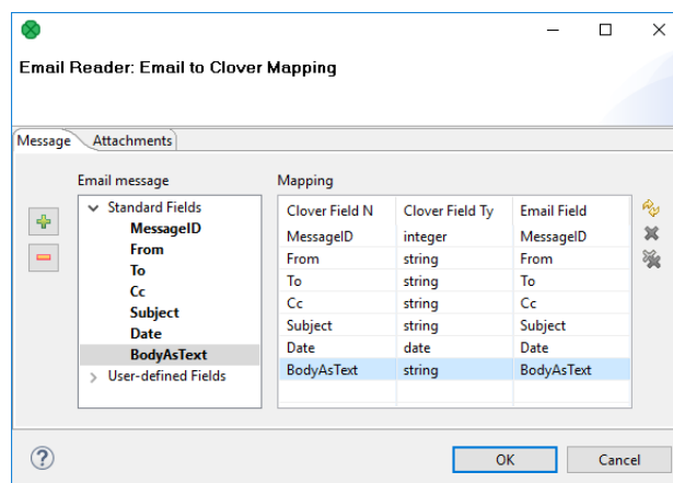
Figure 56.12. Mapping to Clover fields in EmailReader
