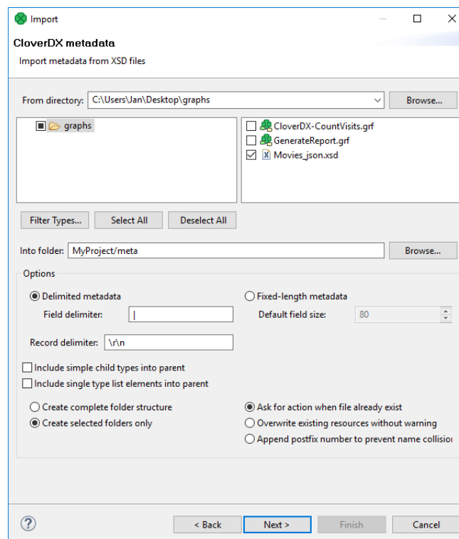
Figure 26.6. Import Metadata from XSD
