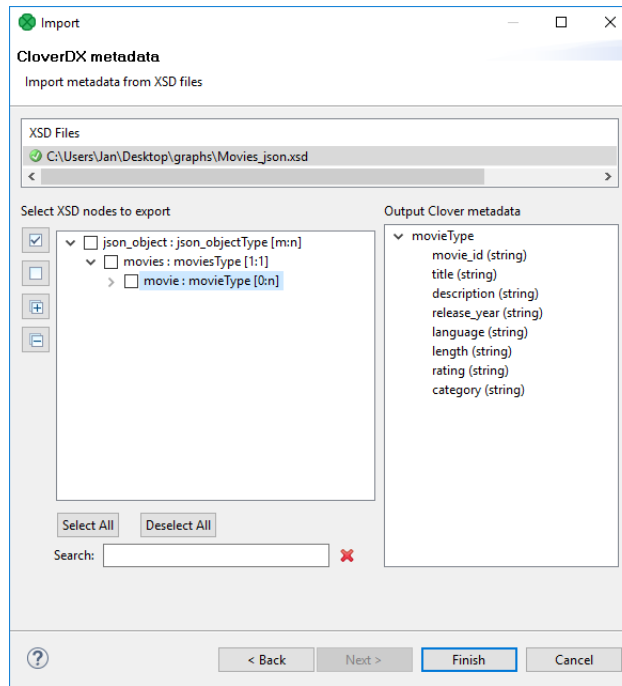
Figure 26.7. Import Metadata from XSD - Review
