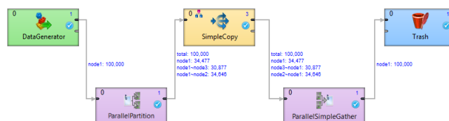
Figure 28.3. An example of a high level tracking information
