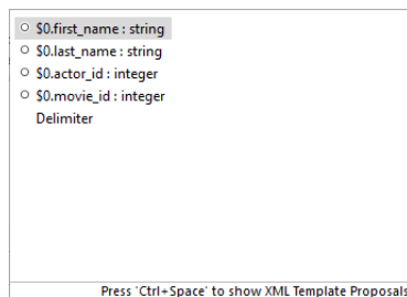
Figure 57.37. Content Assist for ports and fields
