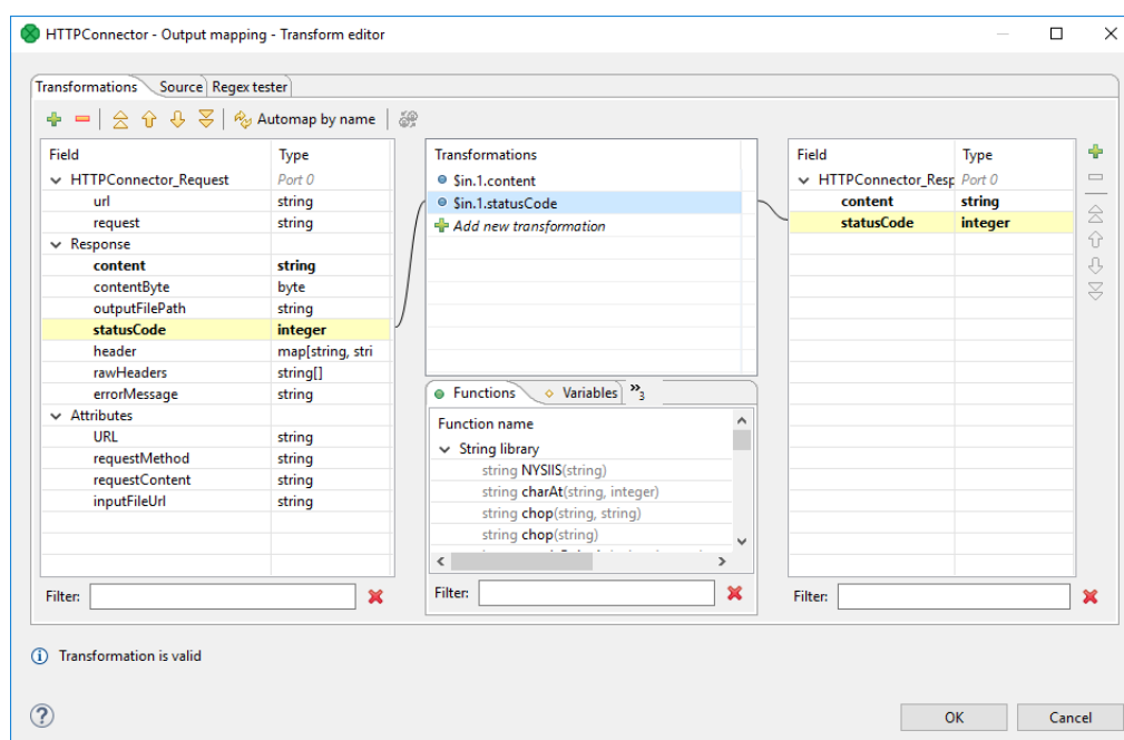
Figure 64.6. Transform Editor in HTTPConnector
