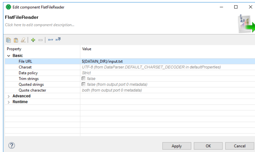
Figure 23.11. Input File URL Attribute Has Been Set
