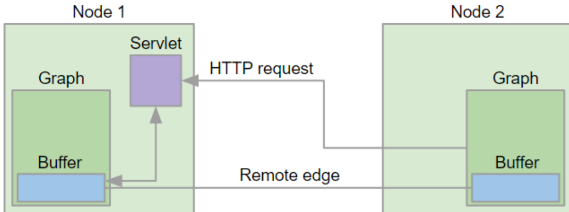
Figure 40.4. Remote Edge Implementation
