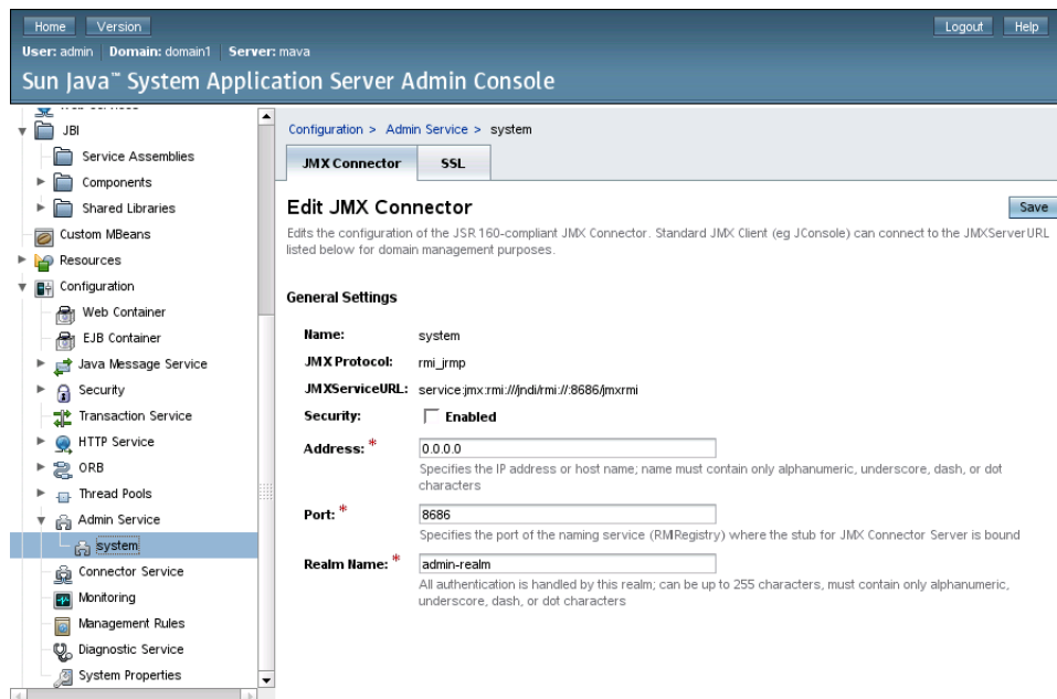
Figure 37.1. Glassfish JMX connector
