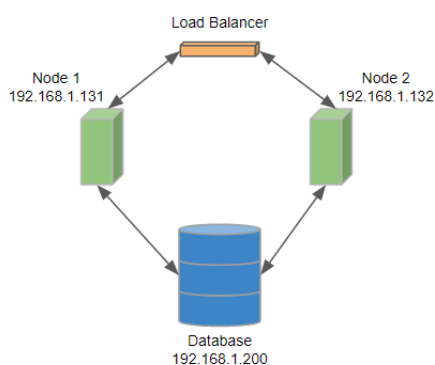
Figure 41.3. Configuration of 2-nodes Cluster with load balancer
