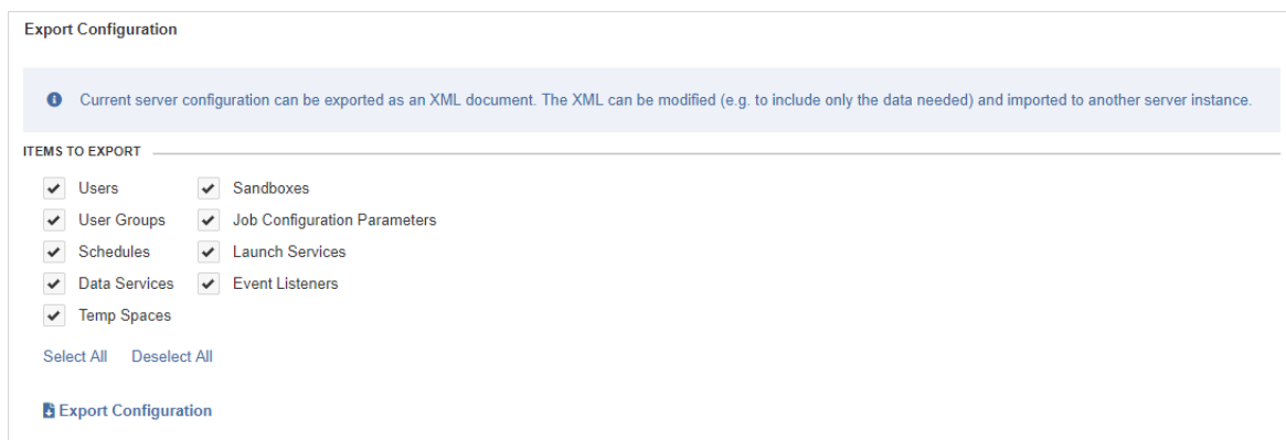
Figure 23.1. Server Configuration Export screen
